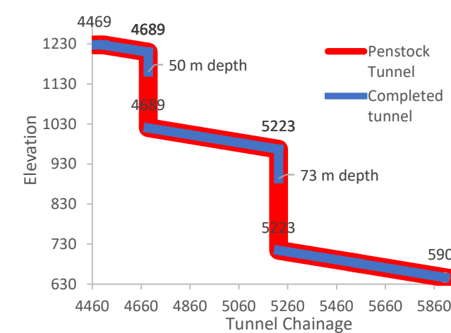
Figure 5. Penstock tunnel progress
