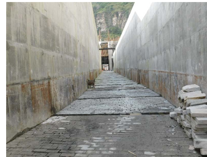
2. Hardstone lining at bedload sluice area
