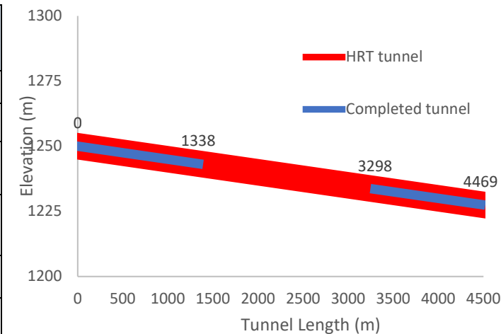
Figure 4. Headrace tunnel progress
