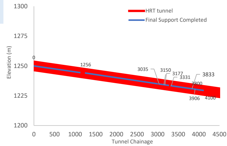
Figure 4. Progress at headrace tunnel
