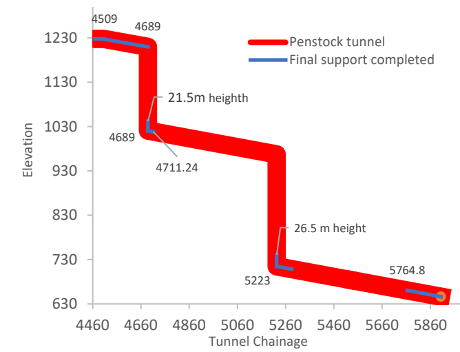
Figure 5. Progress at Penstock tunnel
