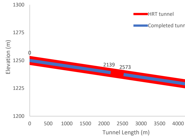
Figure 4. Headrace tunnel progress
