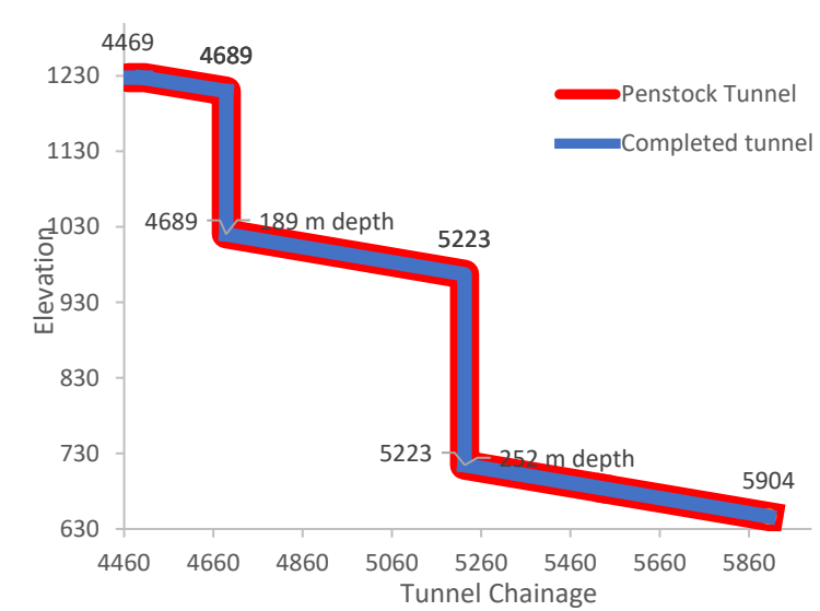
Figure 5. Penstock tunnel
