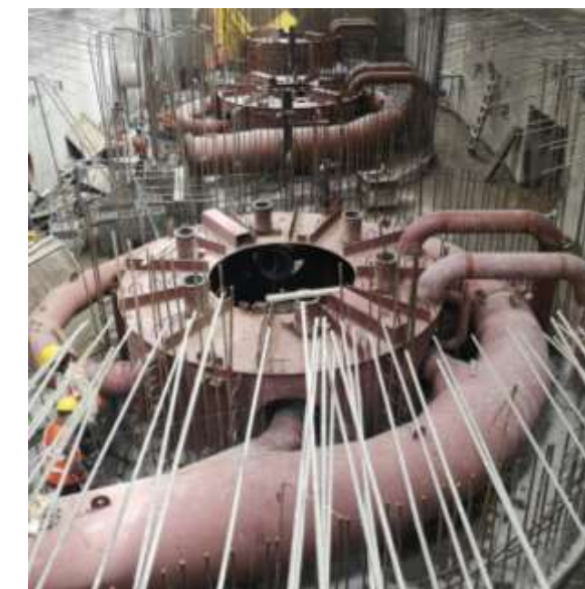
7. Turbine housing assembly and fitting work at Powerhouse
