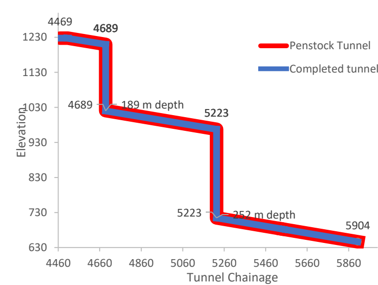
Figure 4. Penstock tunnel progress
